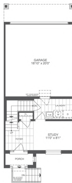
FIRST FLOOR ELEV. A
