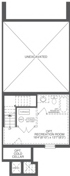
BASEMENT ELEV. A OPT. FINISHED BASEMENT 164 sf
