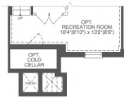
BASEMENT ELEV. A1 BLOCK 3 LOT 10 OPT. FINISHED BASEMENT 172 sf
