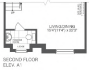
SECOND FLOOR ELEV. A1 (MOD.) BLOCK 3 LOT 10
