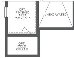
BASEMENT ELEV. B OPT. FINISHED BASEMENT 437 sf
