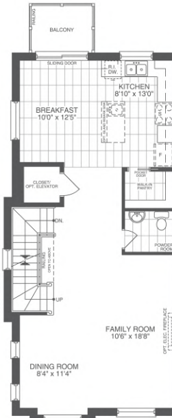
SECOND FLOOR ELEV. A
