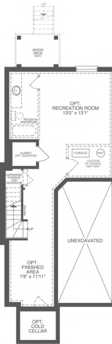
BASEMENT ELEV. A OPT. FINISHED BASEMENT 426 sf
