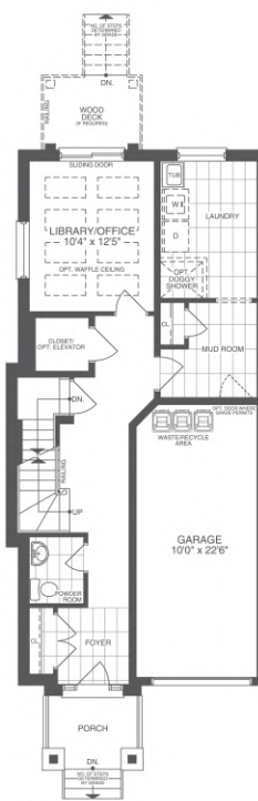
FIRST FLOOR ELEV. A
