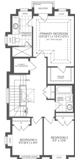
THIRD FLOOR ELEV. B BLOCK 8 LOT 35
