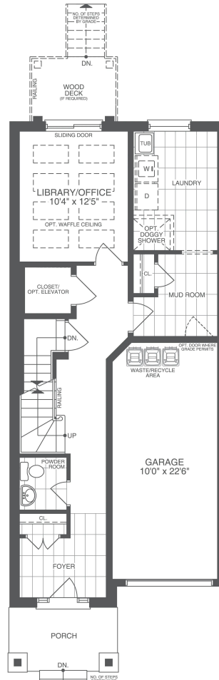
FIRST FLOOR ELEV. A
