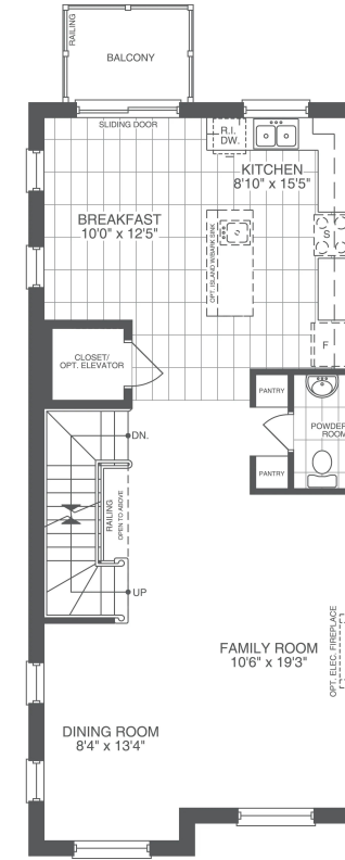
SECOND FLOOR ELEV. A
