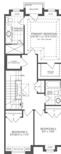
THIRD FLOOR ELEV. A
