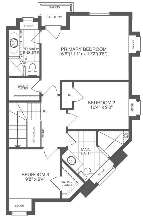
THIRD FLOOR ELEV. B
