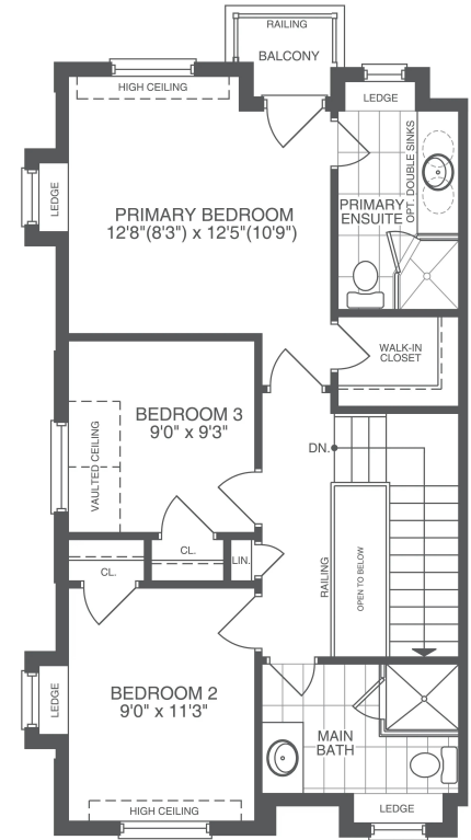
THIRD FLOOR ELEV. C BLOCK 1 LOT 1
